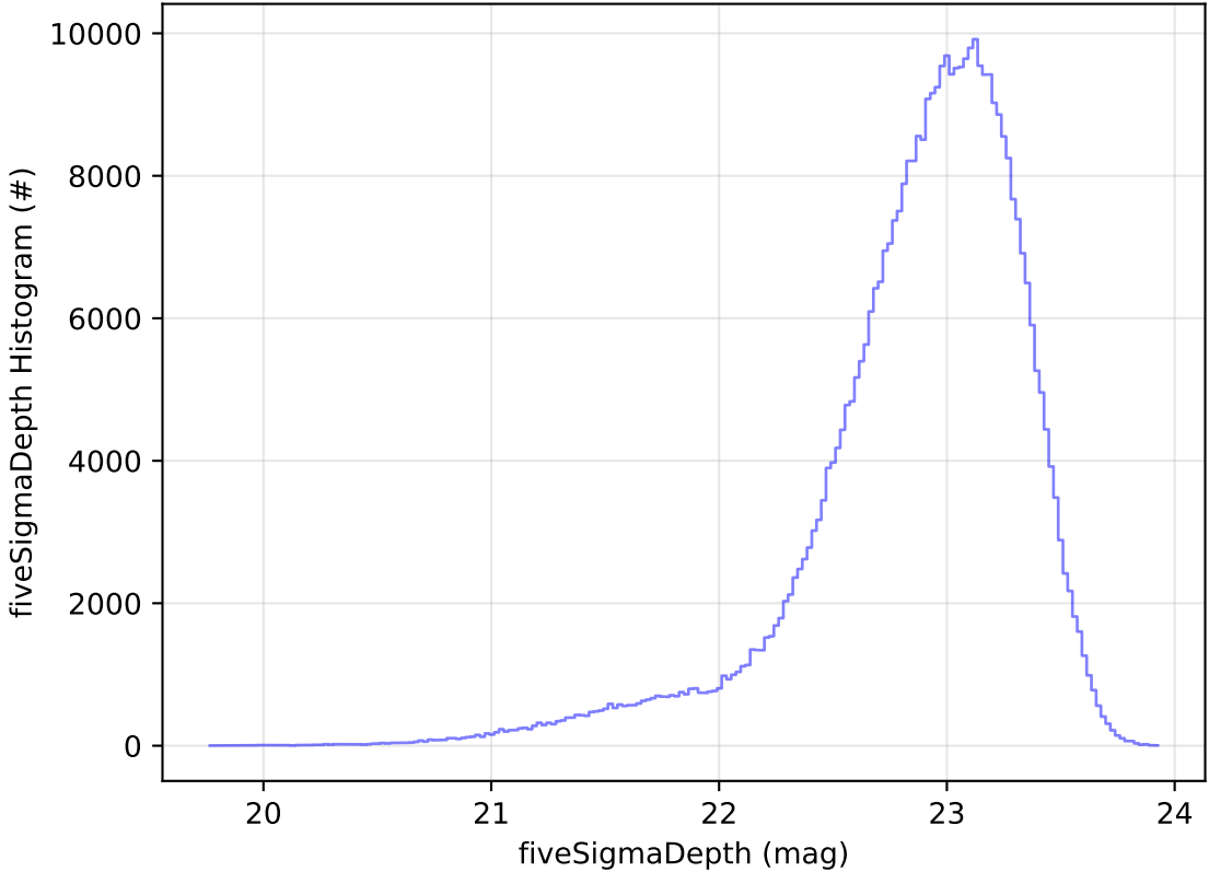
too_elab_2yr_r128_d3_griz_v3.4_10yrs WFD z band: fiveSigmaDepth Histogram
