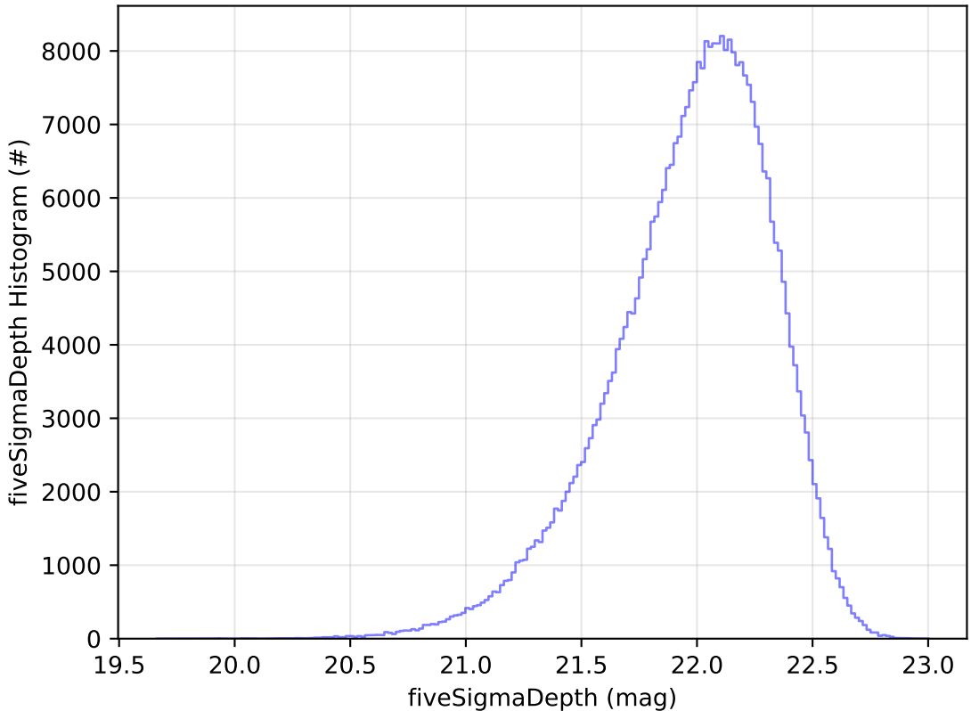
too_elab_2yr_r128_d3_griz_v3.4_10yrs WFD y band: fiveSigmaDepth Histogram
