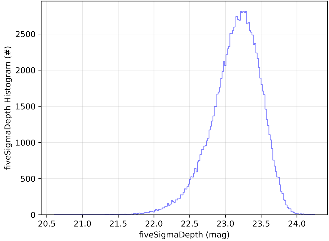
too_elab_2yr_r128_d3_griz_v3.4_10yrs WFD u band: fiveSigmaDepth Histogram
