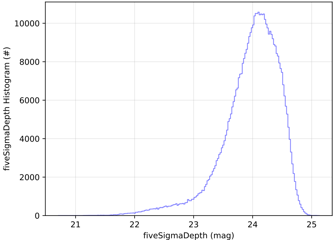
too_elab_2yr_r128_d3_griz_v3.4_10yrs WFD r band: fiveSigmaDepth Histogram
