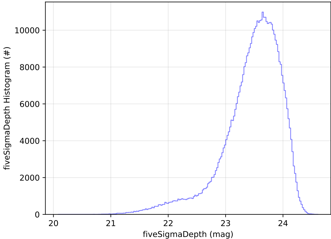
too_elab_2yr_r128_d3_griz_v3.4_10yrs WFD i band: fiveSigmaDepth Histogram
