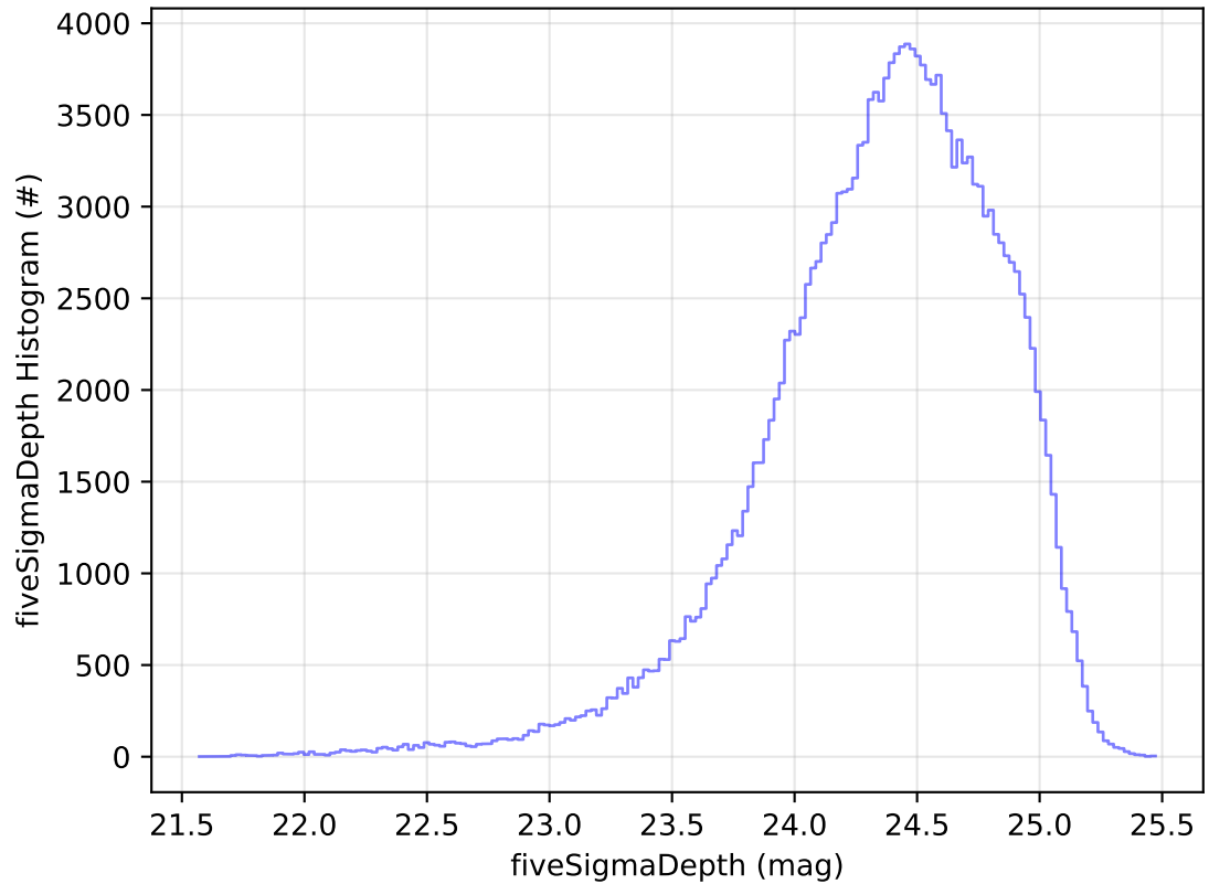
too_elab_2yr_r128_d3_griz_v3.4_10yrs WFD g band: fiveSigmaDepth Histogram
