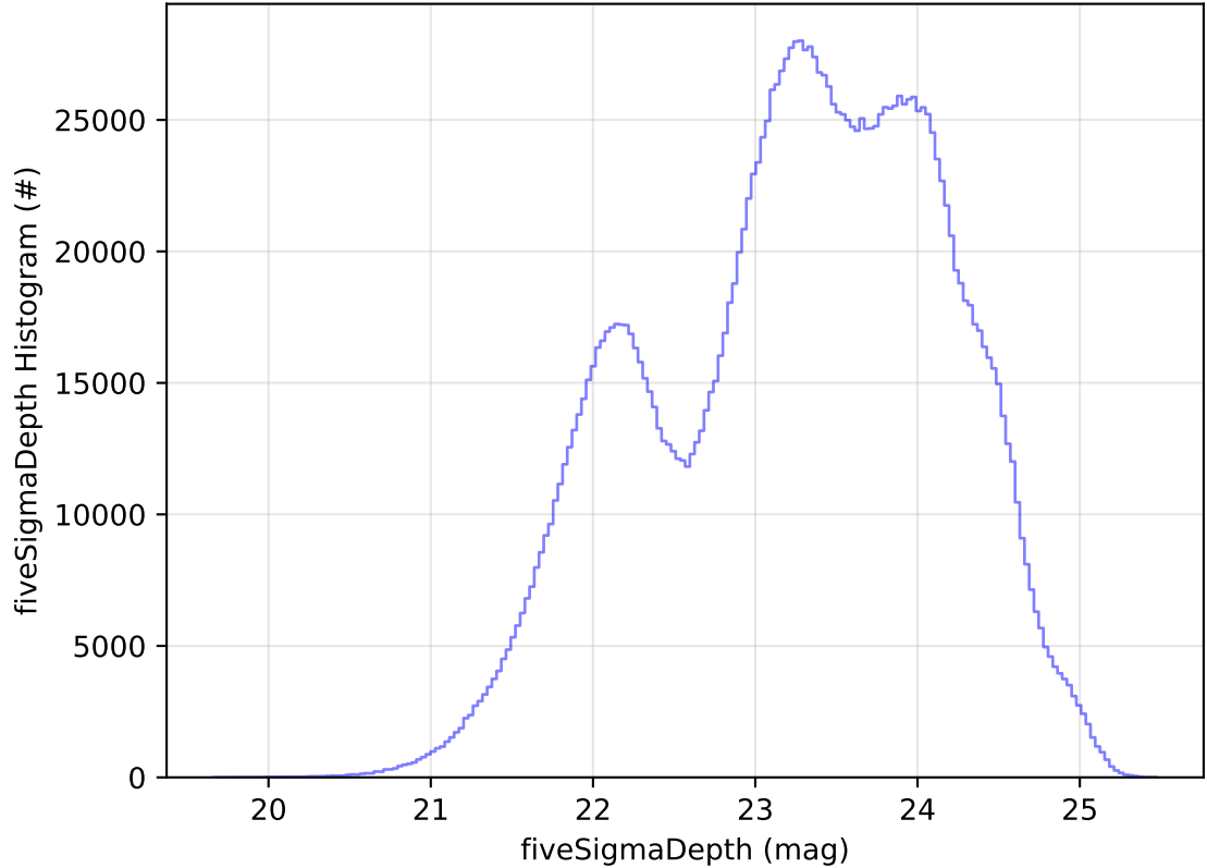
too_elab_2yr_r128_d3_griz_v3.4_10yrs WFD all bands: fiveSigmaDepth Histogram
