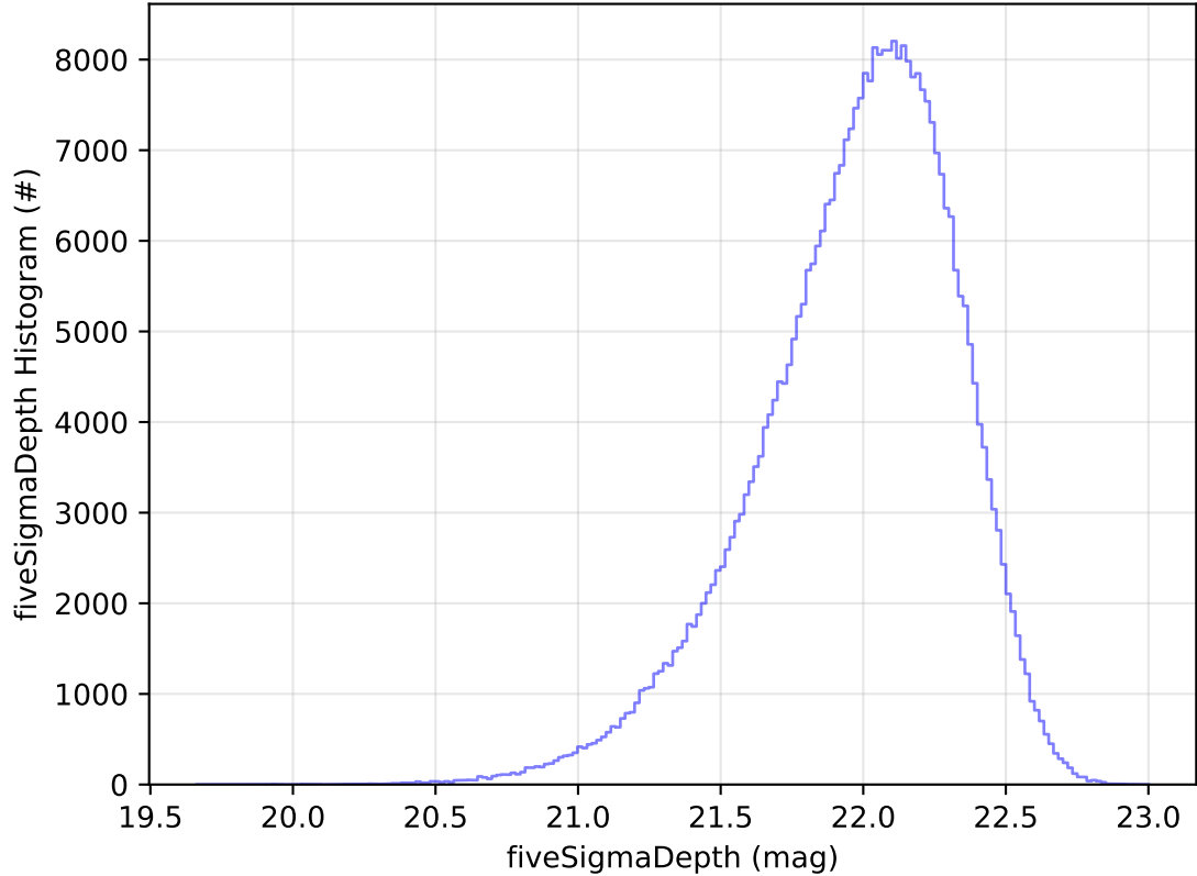
too_elab_2yr_r128_d3_griz_v3.4_10yrs All sky y band: fiveSigmaDepth Histogram
