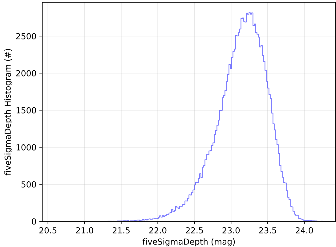
too_elab_2yr_r128_d3_griz_v3.4_10yrs All sky u band: fiveSigmaDepth Histogram
