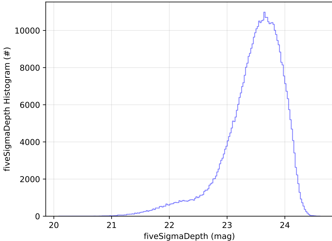
too_elab_2yr_r128_d3_griz_v3.4_10yrs All sky i band: fiveSigmaDepth Histogram
