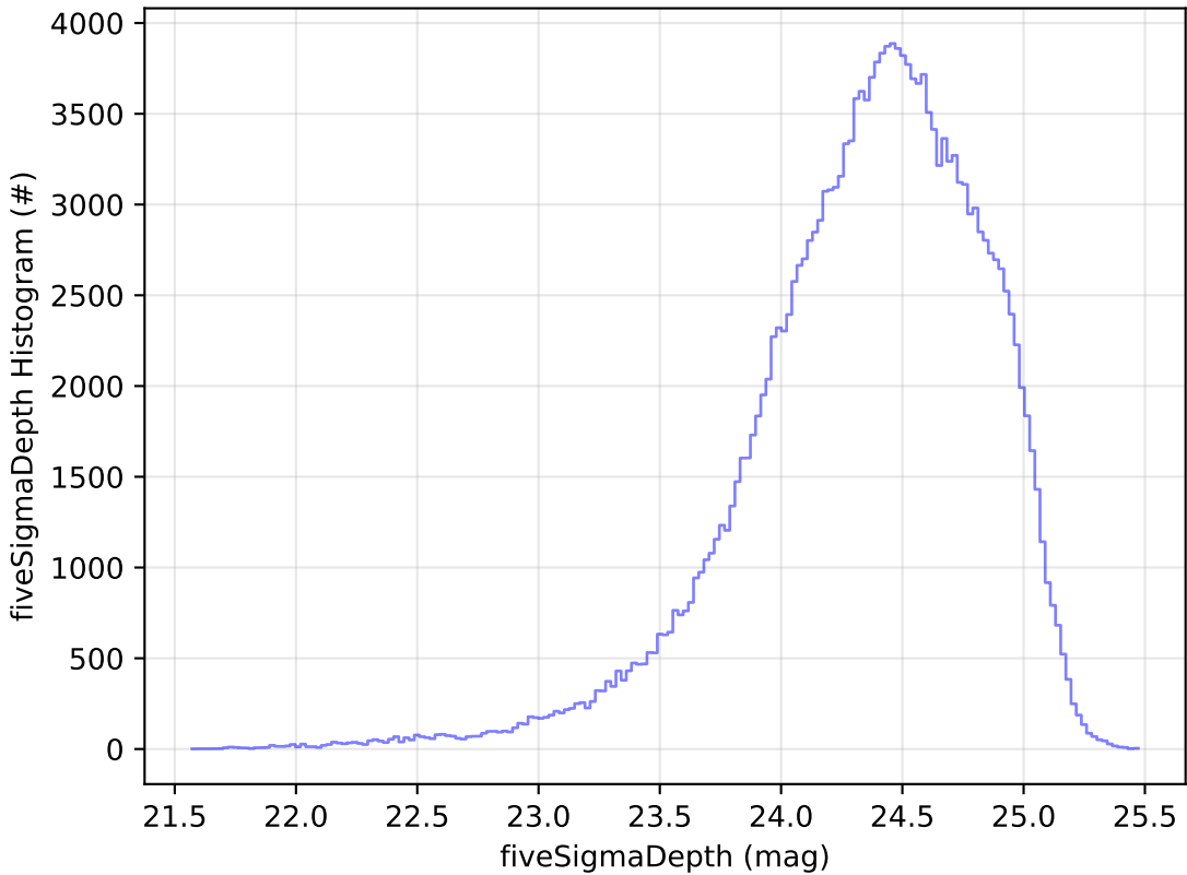
too_elab_2yr_r128_d3_griz_v3.4_10yrs All sky g band: fiveSigmaDepth Histogram
