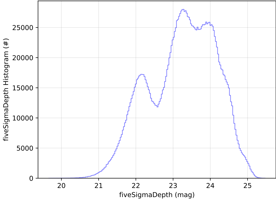
too_elab_2yr_r128_d3_griz_v3.4_10yrs All sky all bands: fiveSigmaDepth Histogram
