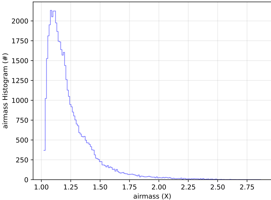
too_elab_2yr_r128_d3_griz_v3.4_10yrs Yr 1 y band: airmass Histogram
