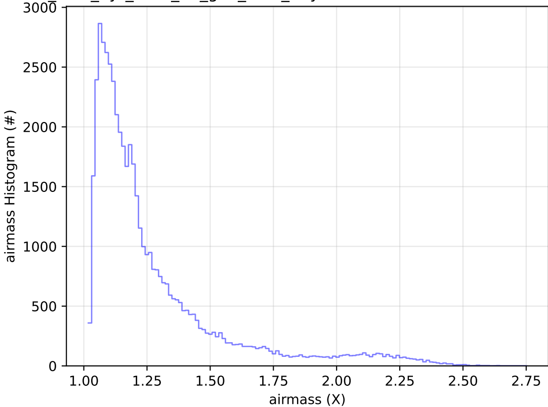
too_elab_2yr_r128_d3_griz_v3.4_10yrs Yr 1 r band: airmass Histogram
