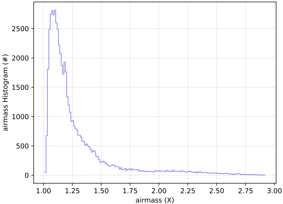
too_elab_2yr_r128_d3_griz_v3.4_10yrs Yr 1 i band: airmass Histogram
