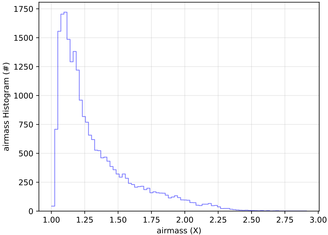
too_elab_2yr_r128_d3_griz_v3.4_10yrs Yr 1 g band: airmass Histogram
