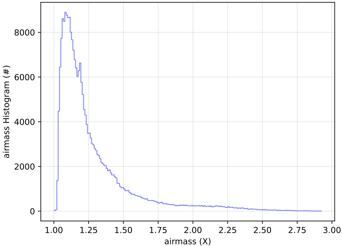
too_elab_2yr_r128_d3_griz_v3.4_10yrs Yr 1 all bands: airmass Histogram
