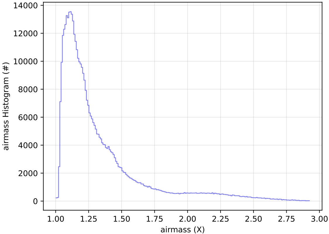
too_elab_2yr_r128_d3_griz_v3.4_10yrs WFD z band: airmass Histogram
