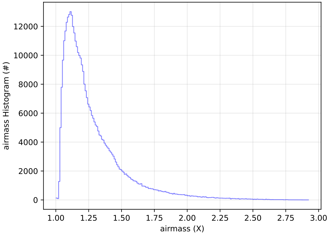
too_elab_2yr_r128_d3_griz_v3.4_10yrs WFD y band: airmass Histogram
