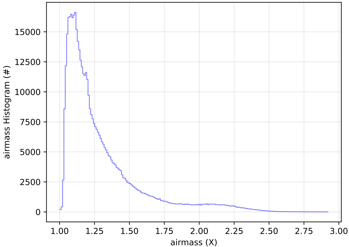
too_elab_2yr_r128_d3_griz_v3.4_10yrs WFD r band: airmass Histogram
