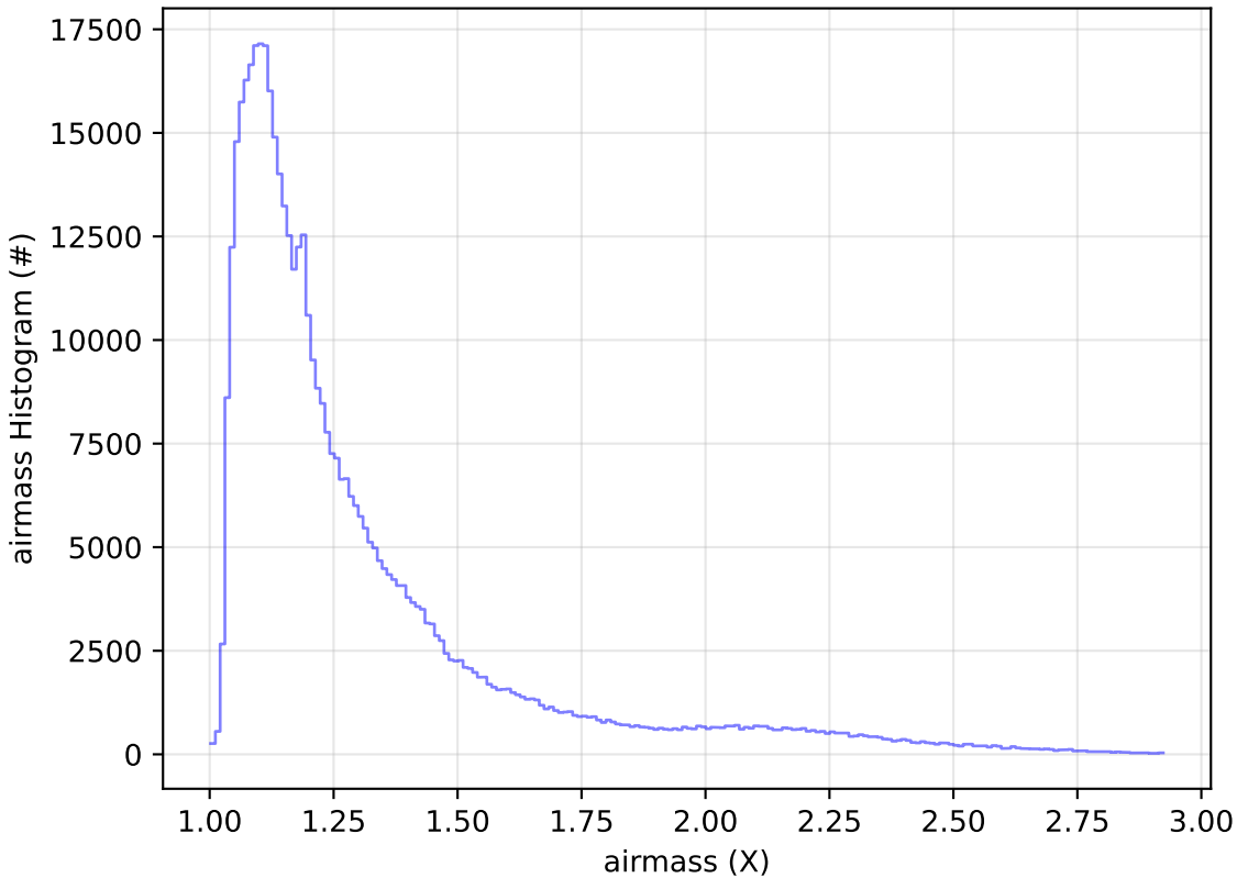
too_elab_2yr_r128_d3_griz_v3.4_10yrs WFD i band: airmass Histogram
