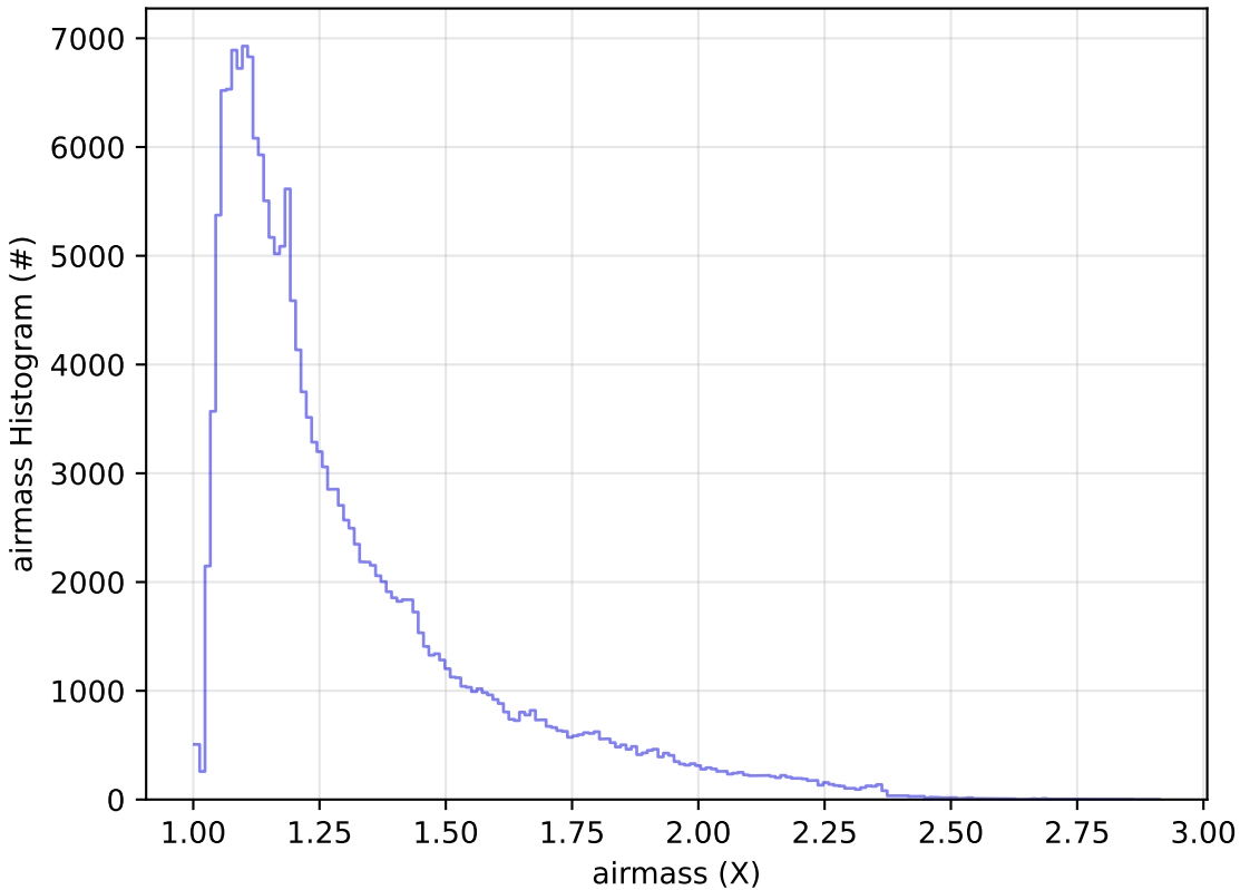
too_elab_2yr_r128_d3_griz_v3.4_10yrs WFD g band: airmass Histogram
