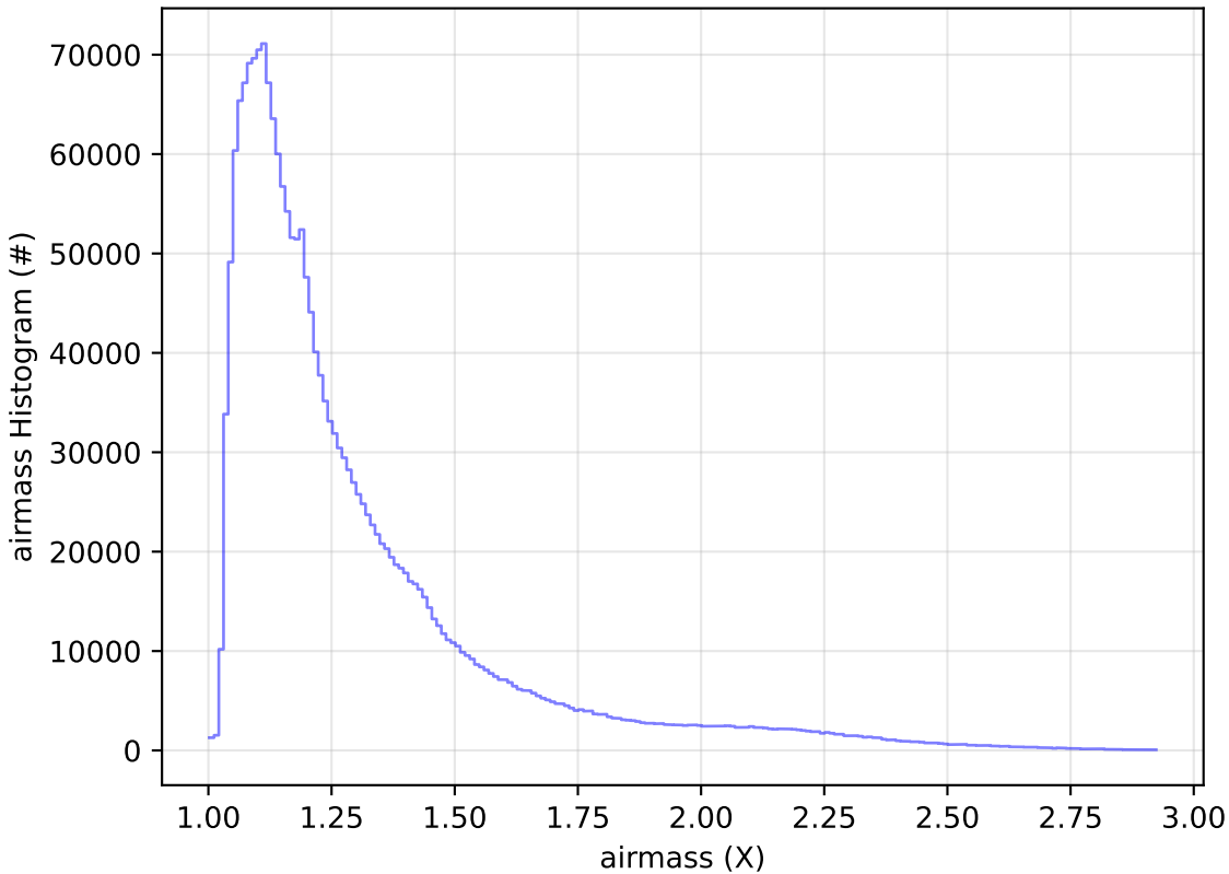
too_elab_2yr_r128_d3_griz_v3.4_10yrs WFD all bands: airmass Histogram
