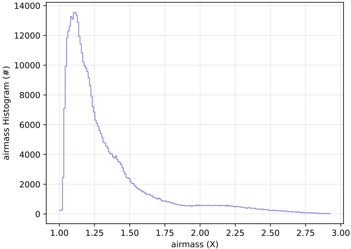
too_elab_2yr_r128_d3_griz_v3.4_10yrs All sky z band: airmass Histogram
