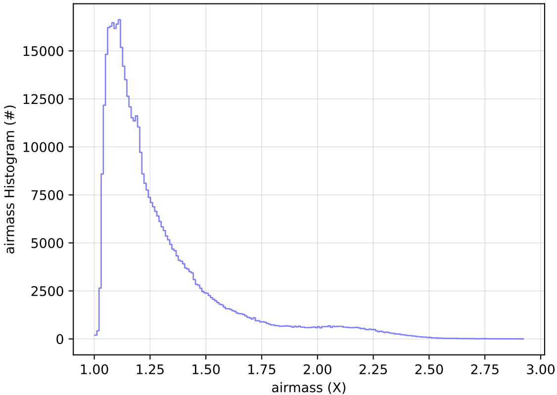
too_elab_2yr_r128_d3_griz_v3.4_10yrs All sky r band: airmass Histogram
