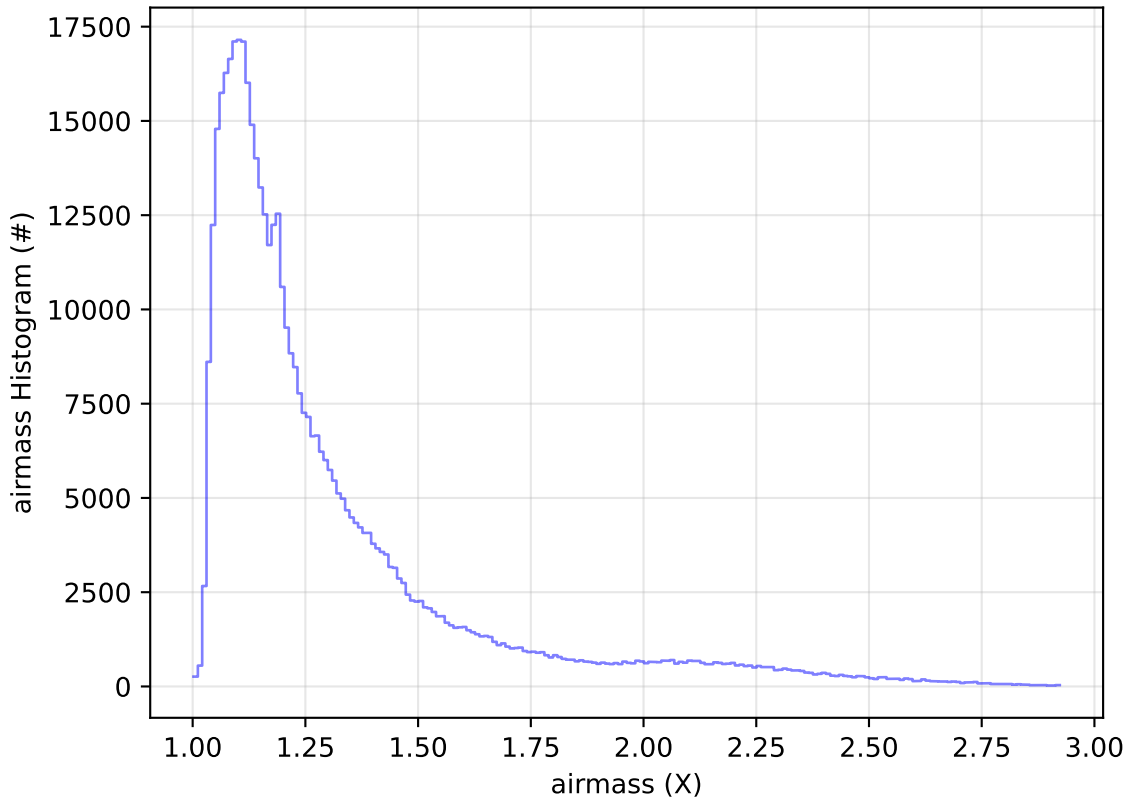
too_elab_2yr_r128_d3_griz_v3.4_10yrs All sky i band: airmass Histogram
