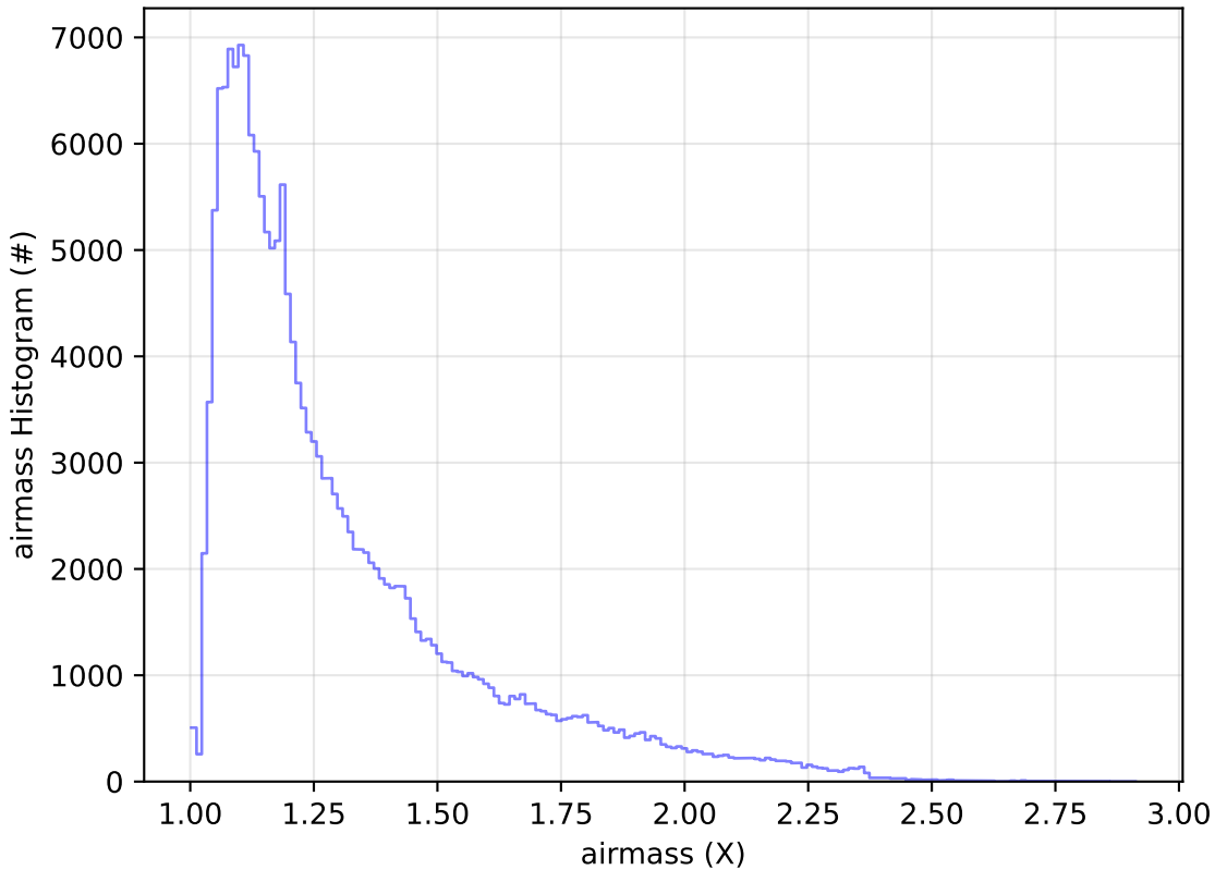
too_elab_2yr_r128_d3_griz_v3.4_10yrs All sky g band: airmass Histogram
