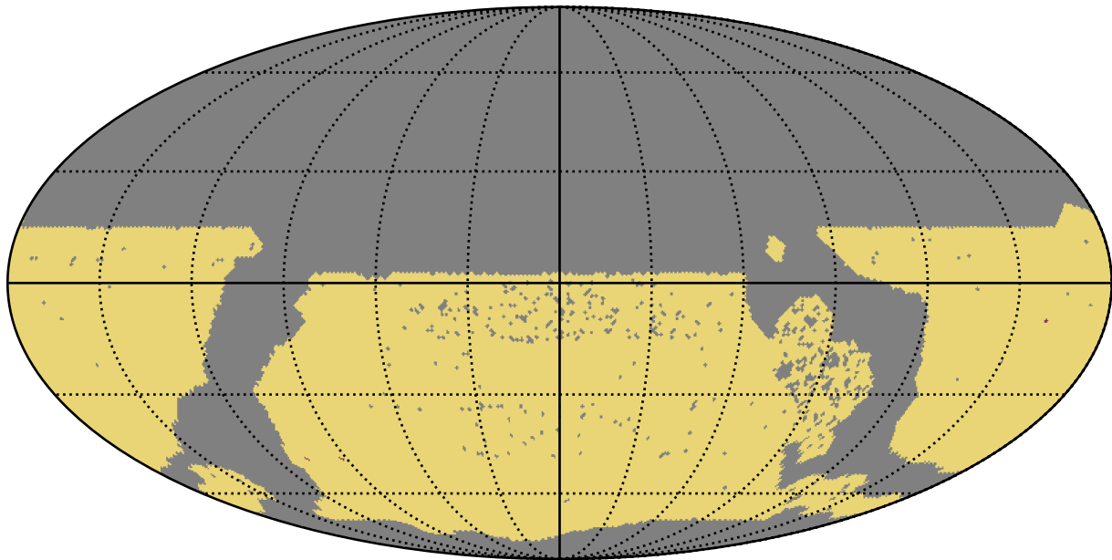
too_elab_2yr_r128_d3_griz_v3.4_10yrs WFD: RapidRevisits
