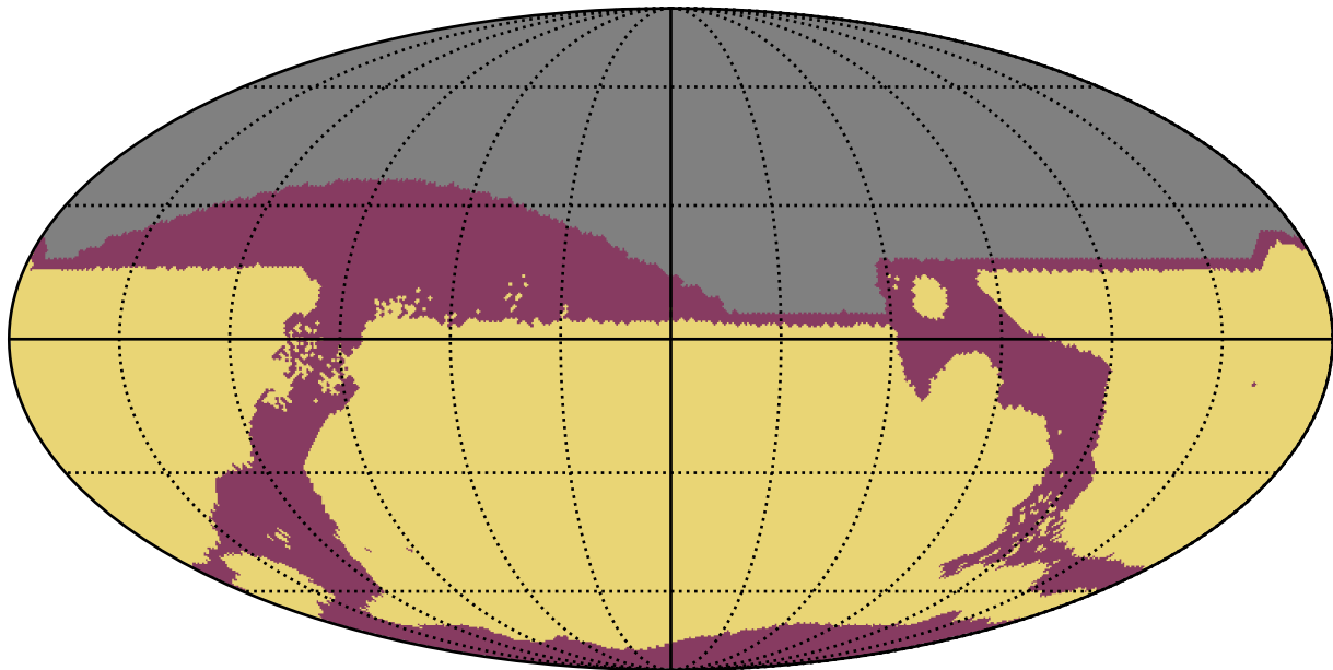
too_elab_2yr_r128_d3_griz_v3.4_10yrs All sky: RapidRevisits
