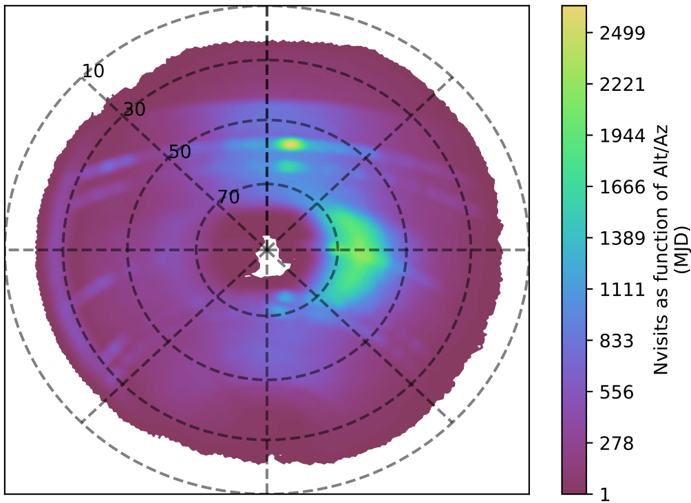
too_elab_2yr_r128_d3_griz_v3.4_10yrs r band: Nvisits as function of Alt/Az
