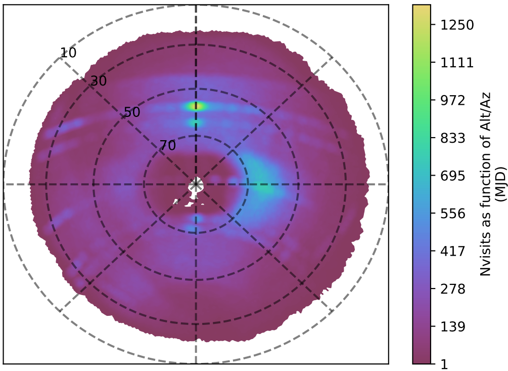
too_elab_2yr_r128_d3_griz_v3.4_10yrs g band: Nvisits as function of Alt/Az
