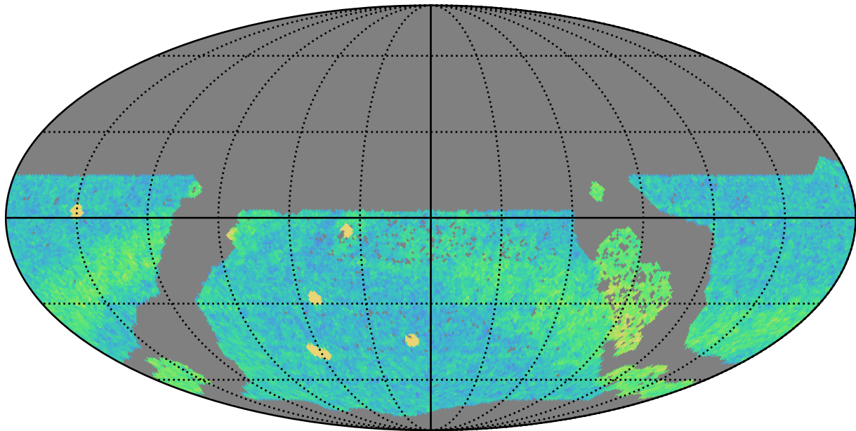
too_elab_2yr_r128_d3_griz_v3.4_10yrs WFD r band: NVisits
