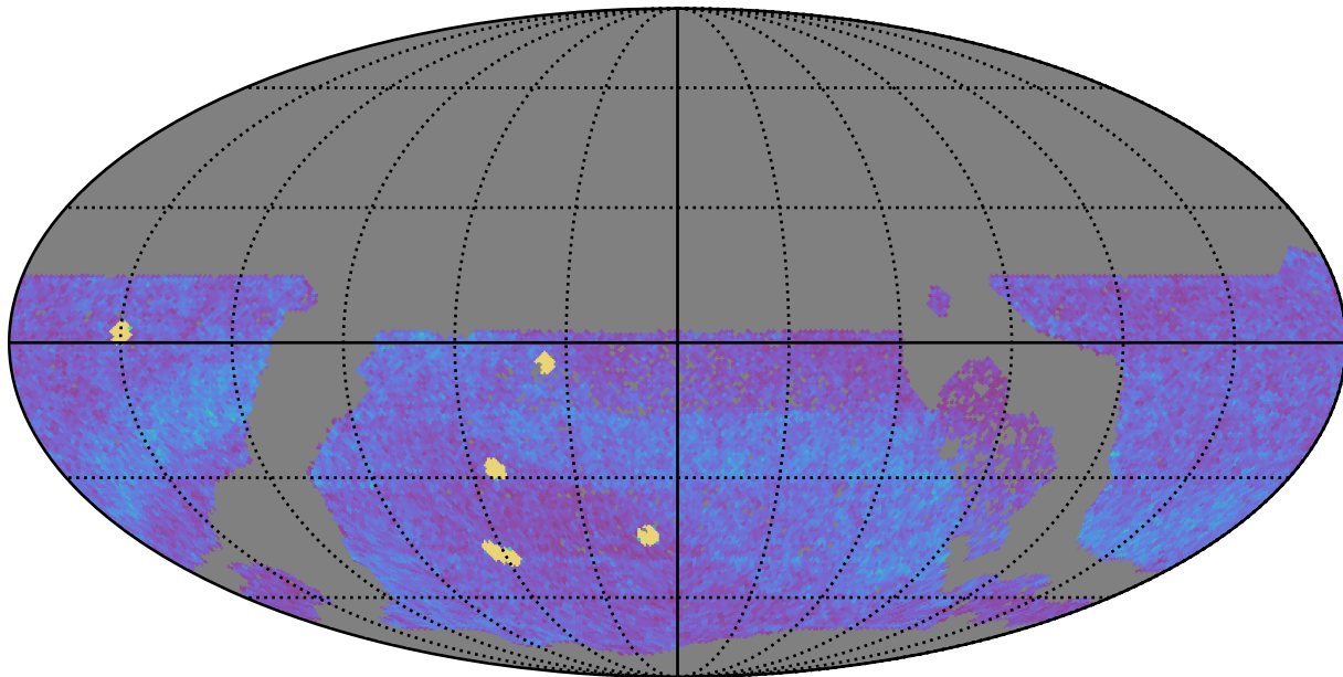
too_elab_2yr_r128_d3_griz_v3.4_10yrs WFD all bands: NVisits
