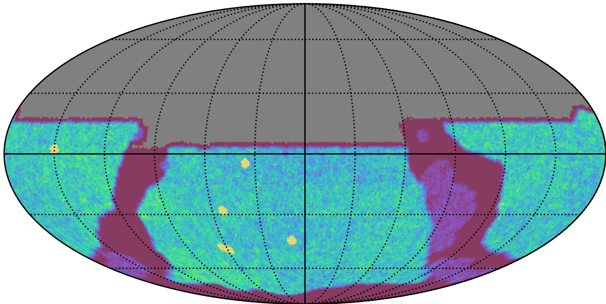
too_elab_2yr_r128_d3_griz_v3.4_10yrs All sky u band: NVisits
