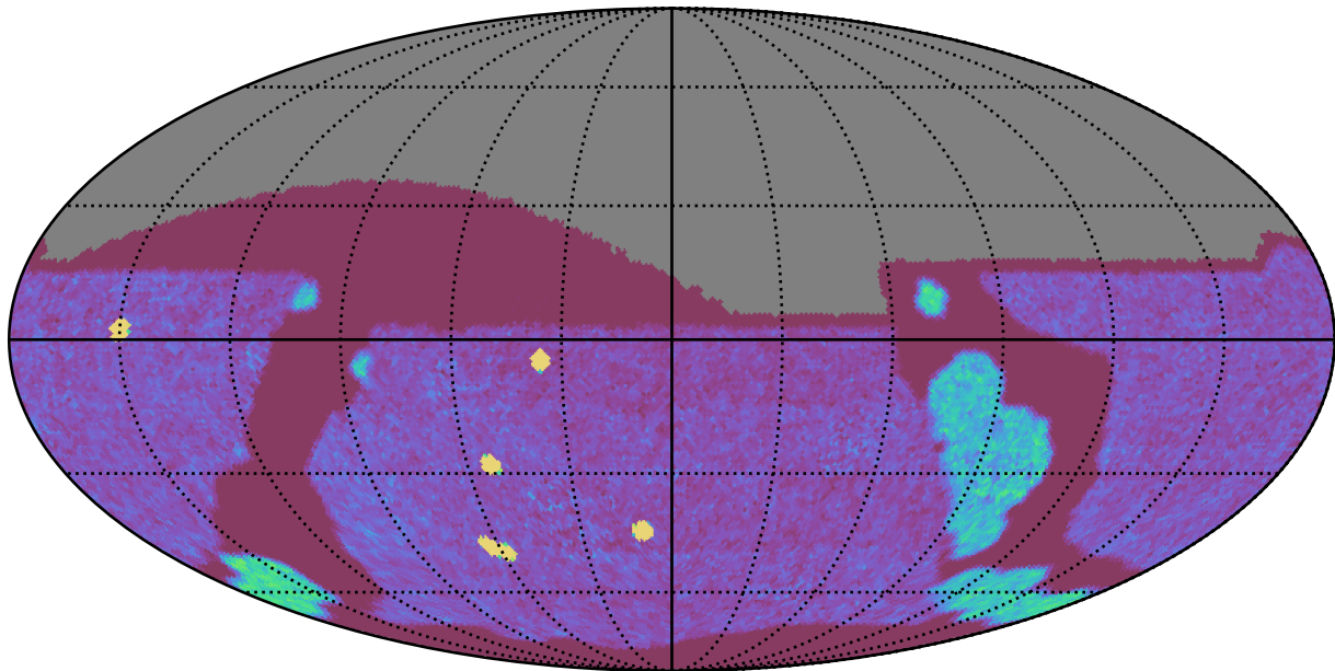
too_elab_2yr_r128_d3_griz_v3.4_10yrs All sky g band: NVisits
