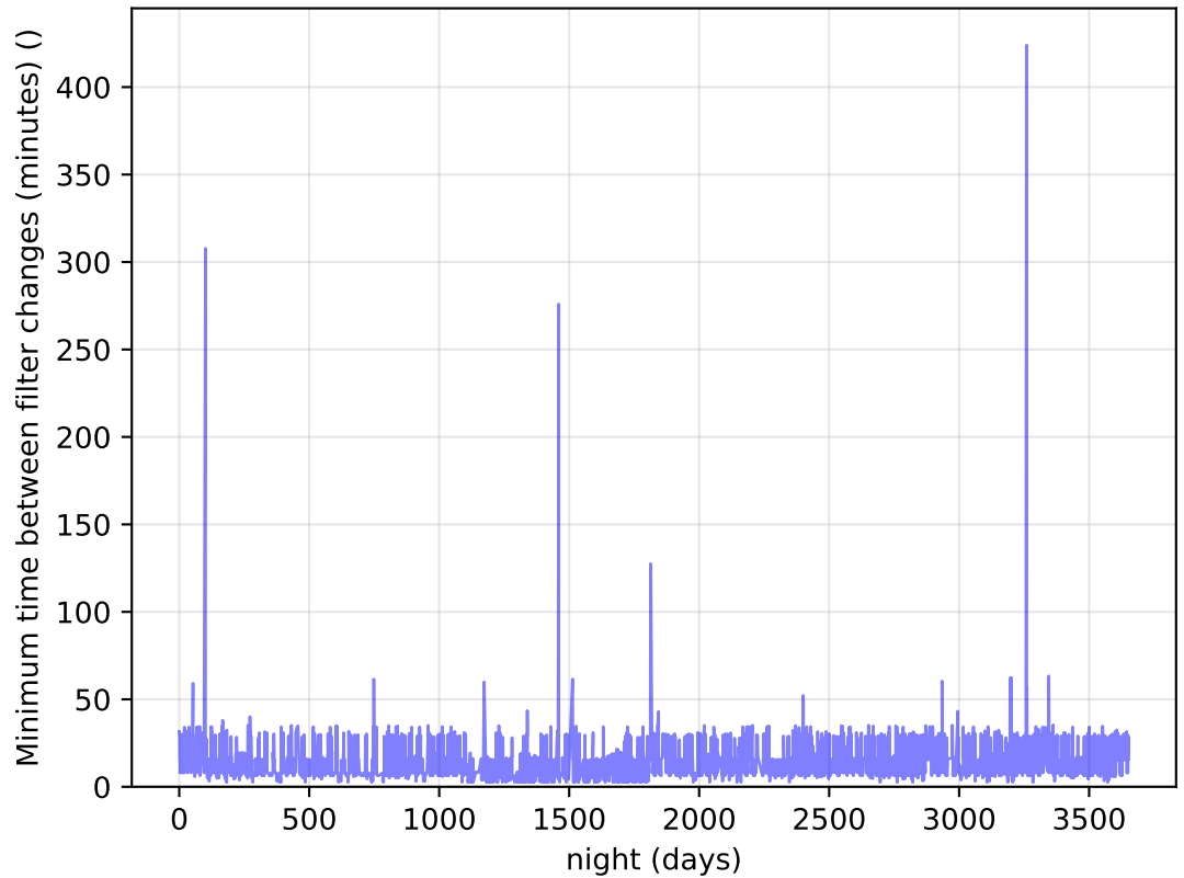
too_elab_2yr_r128_d3_griz_v3.4_10yrs Per Night: Minimum time between filter changes (minutes)
