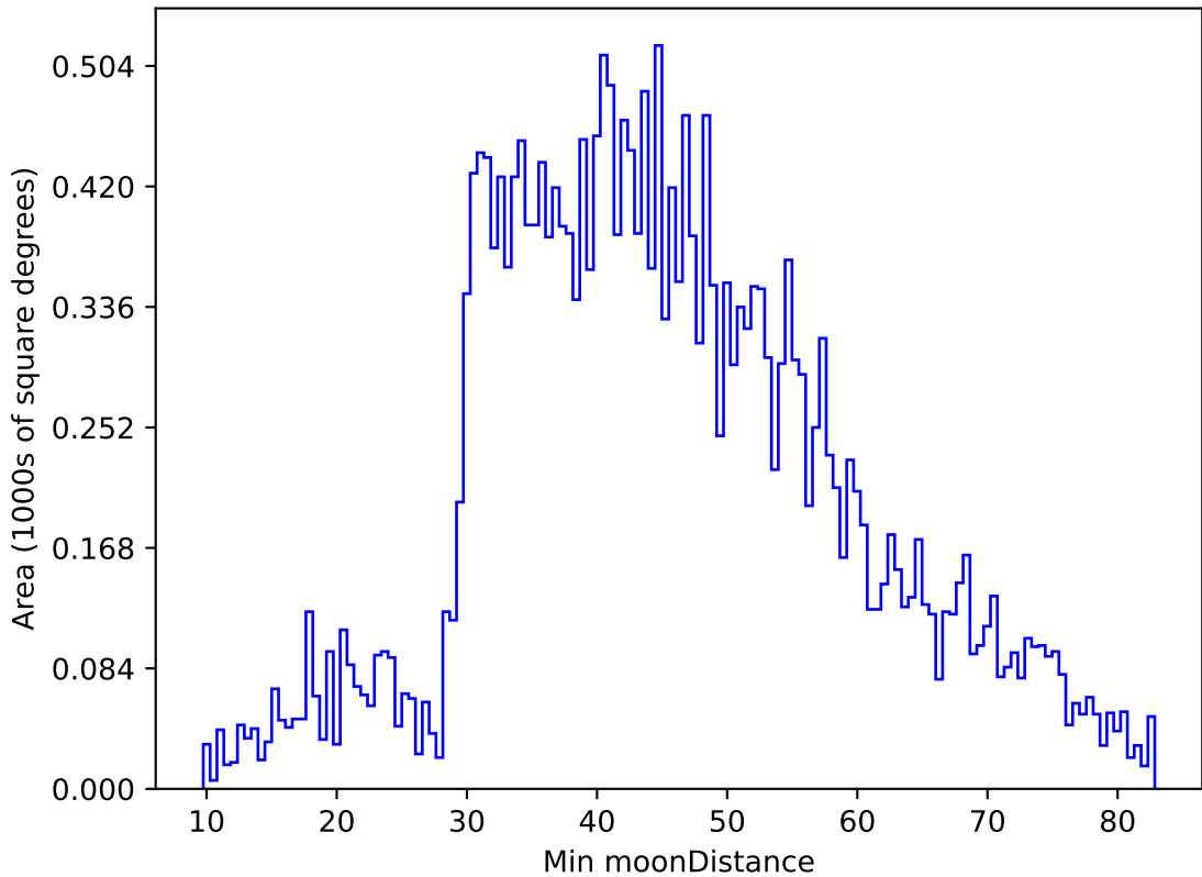
too_elab_2yr_r128_d3_griz_v3.4_10yrs All sky g band: Min moonDistance
