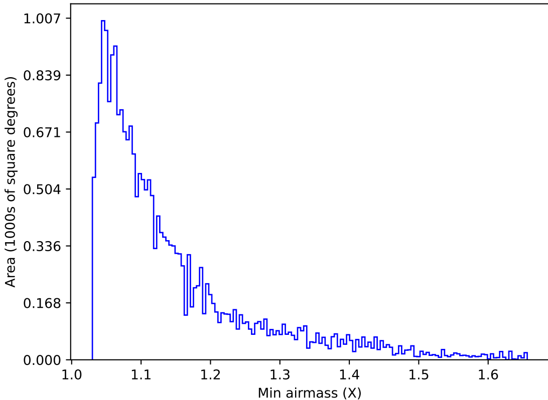
too_elab_2yr_r128_d3_griz_v3.4_10yrs Yr 1 u band: Min airmass
