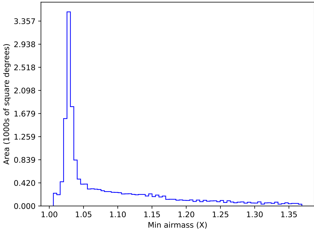
too_elab_2yr_r128_d3_griz_v3.4_10yrs WFD z band: Min airmass
