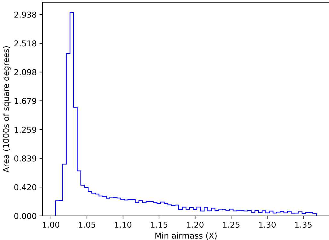
too_elab_2yr_r128_d3_griz_v3.4_10yrs WFD i band: Min airmass
