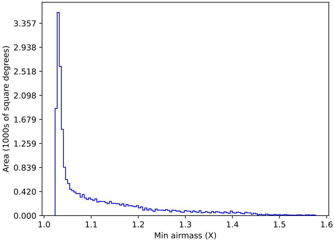
too_elab_2yr_r128_d3_griz_v3.4_10yrs All sky y band: Min airmass
