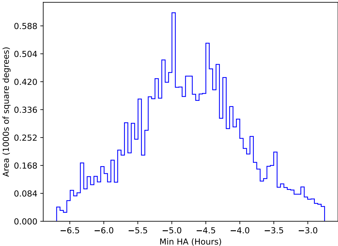
too_elab_2yr_r128_d3_griz_v3.4_10yrs WFD all bands: Min HA
