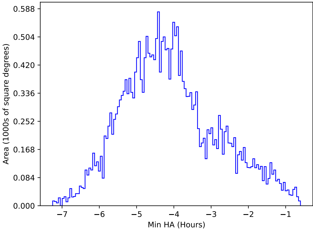
too_elab_2yr_r128_d3_griz_v3.4_10yrs All sky z band: Min HA
