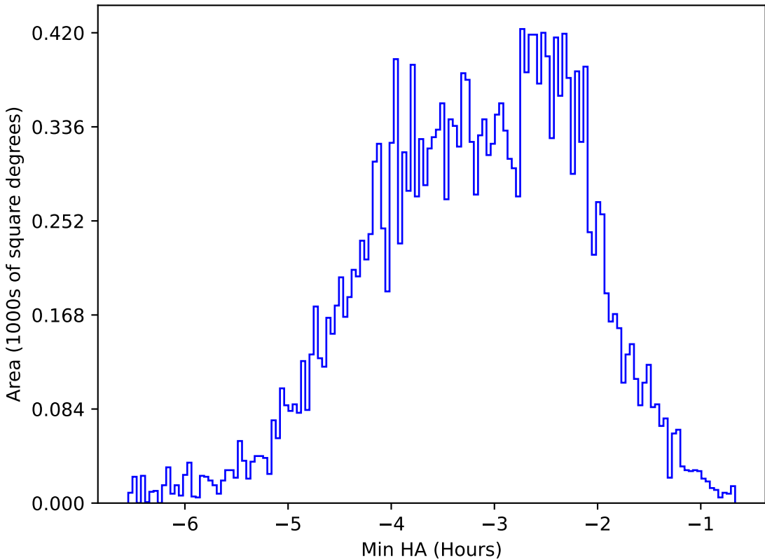
too_elab_2yr_r128_d3_griz_v3.4_10yrs All sky u band: Min HA
