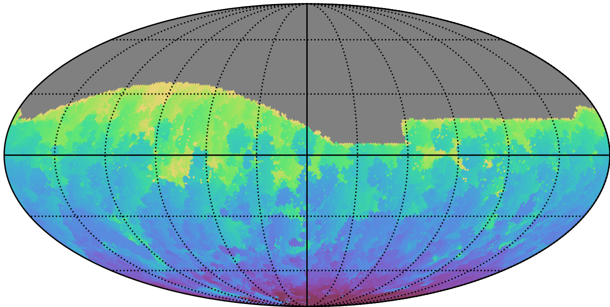
too_elab_2yr_r128_d3_griz_v3.4_10yrs All sky g band: Min HA
