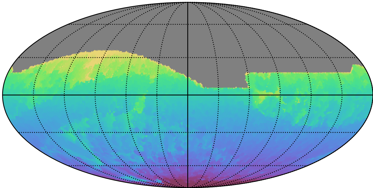
too_elab_2yr_r128_d3_griz_v3.4_10yrs All sky all bands: Min HA
