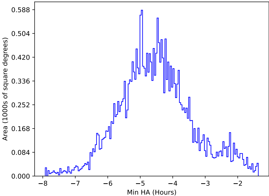
too_elab_2yr_r128_d3_griz_v3.4_10yrs All sky all bands: Min HA
