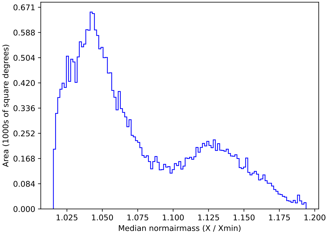
too_elab_2yr_r128_d3_griz_v3.4_10yrs All sky r band: Median normairmass
