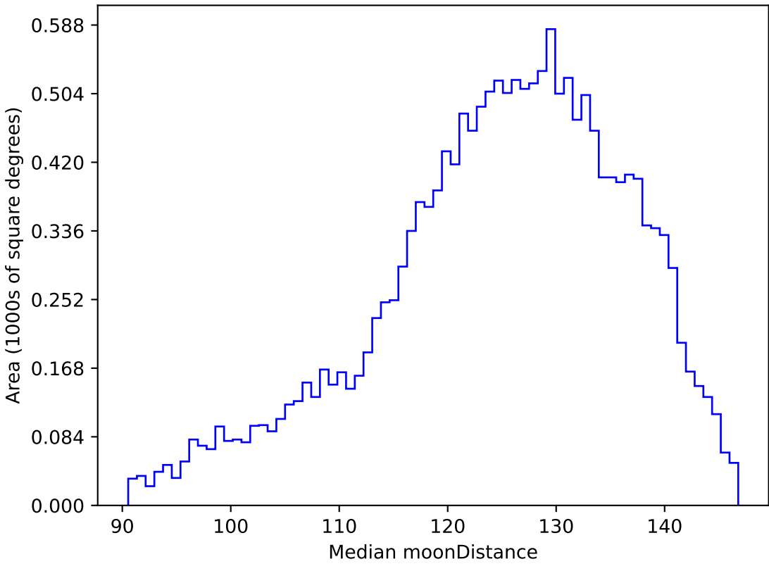
too_elab_2yr_r128_d3_griz_v3.4_10yrs WFD u band: Median moonDistance
