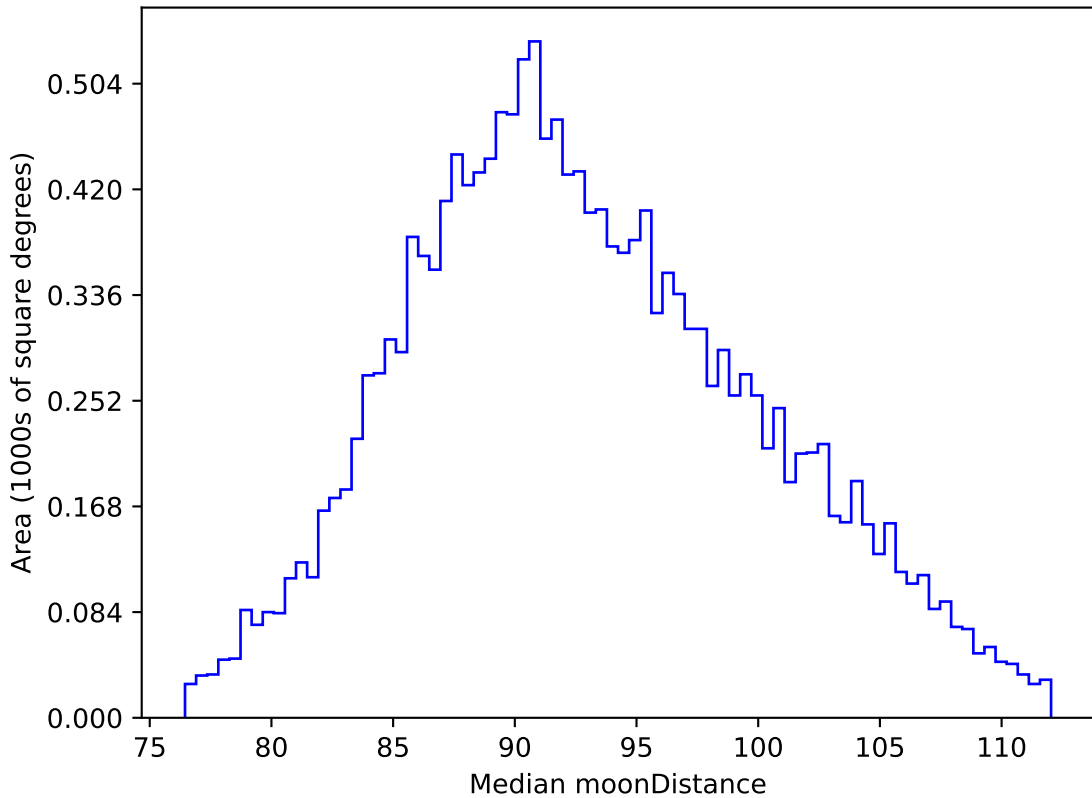
too_elab_2yr_r128_d3_griz_v3.4_10yrs WFD i band: Median moonDistance
